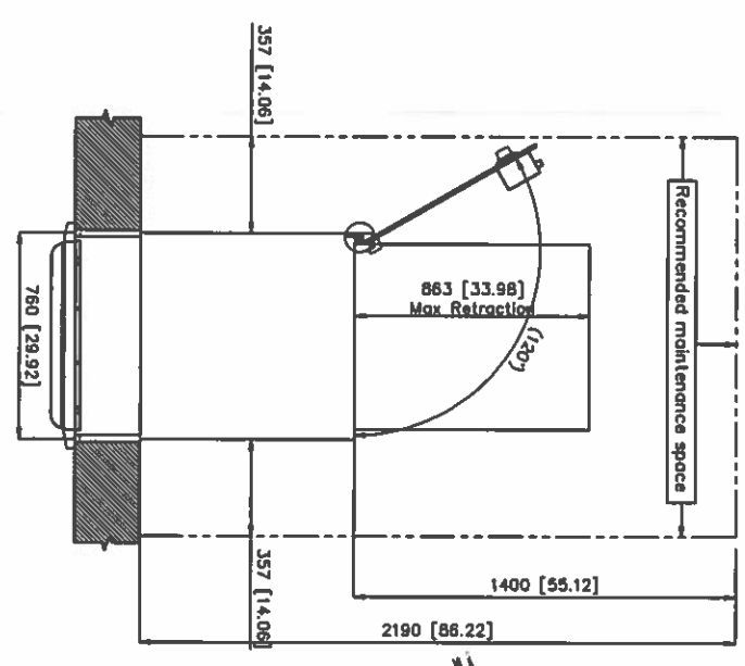
Plane cross-sectional view (RECOMMEND)
