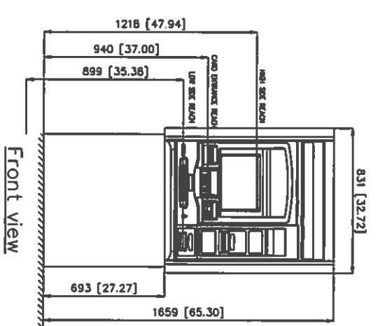
Plane cross-sectional view (RECOMMEND)
