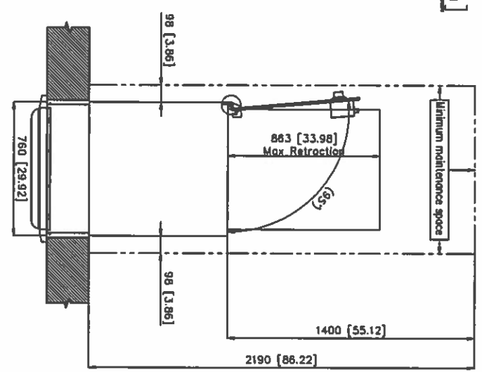
Plane cross-sectional view (MINIMUM)
