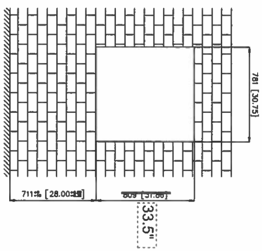
Wall construction plan
